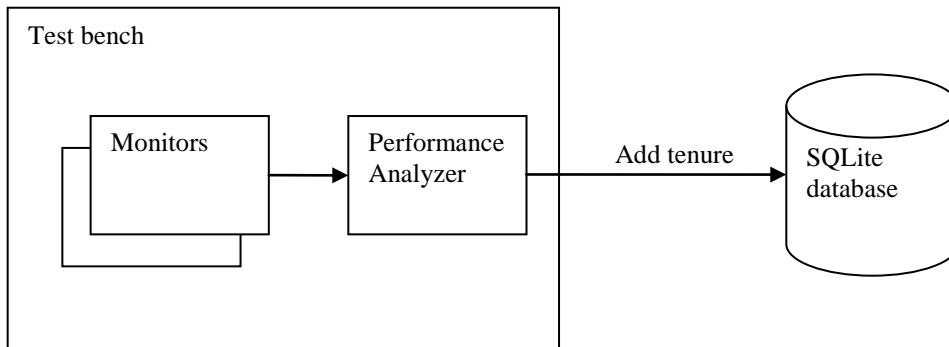
Figure 1 VMM Performance Analyzer - simple implementation
