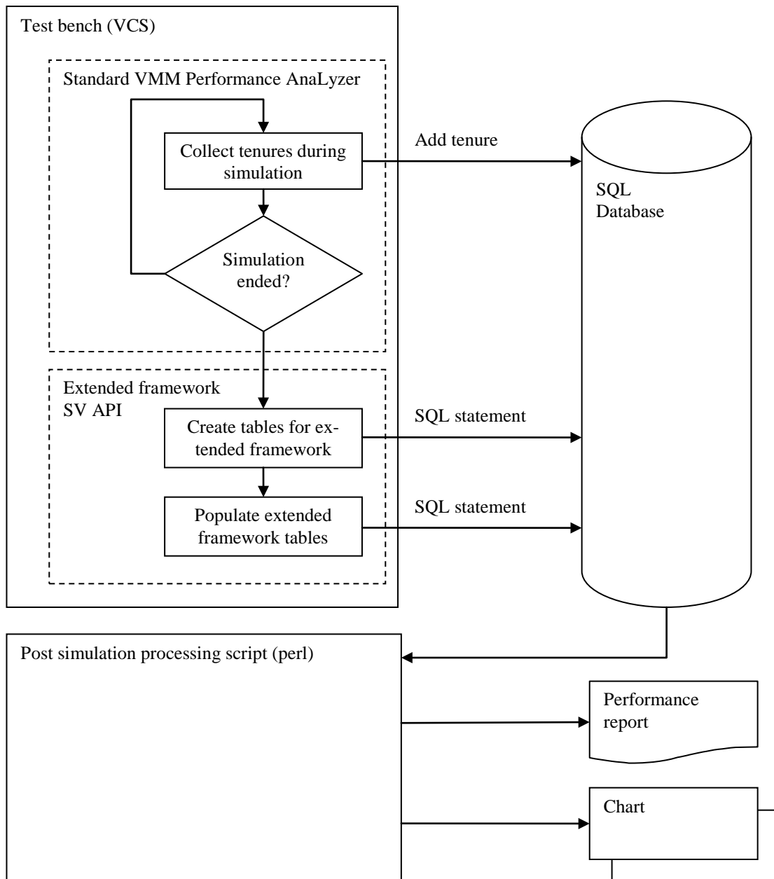
Figure 2 Performance Analyzer Flow
