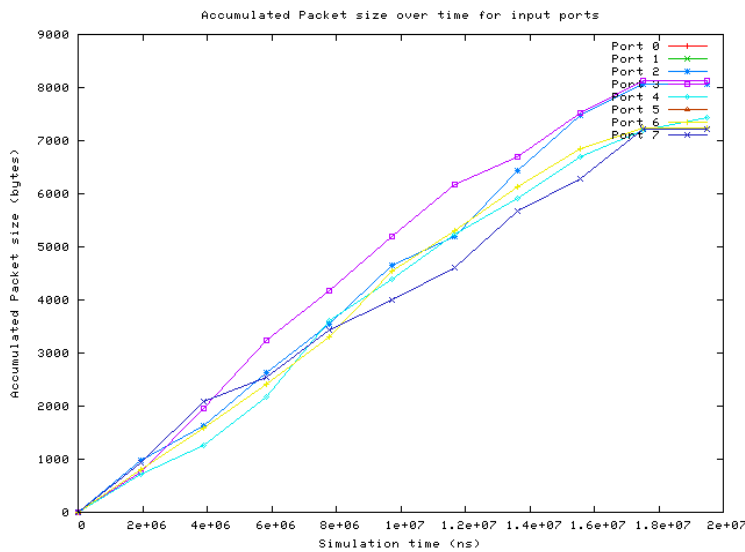
Figure 5 Gnuplot example
