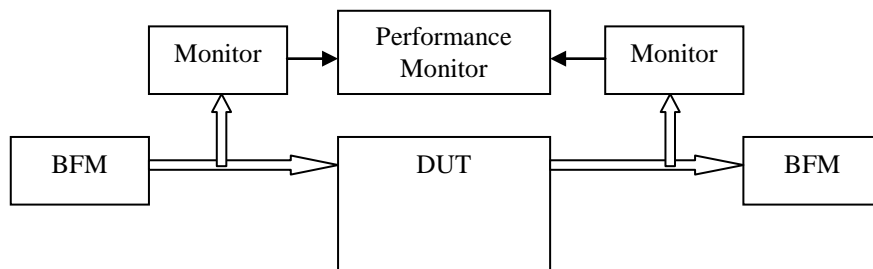
Figure 4 Performance Monitor Implementation
